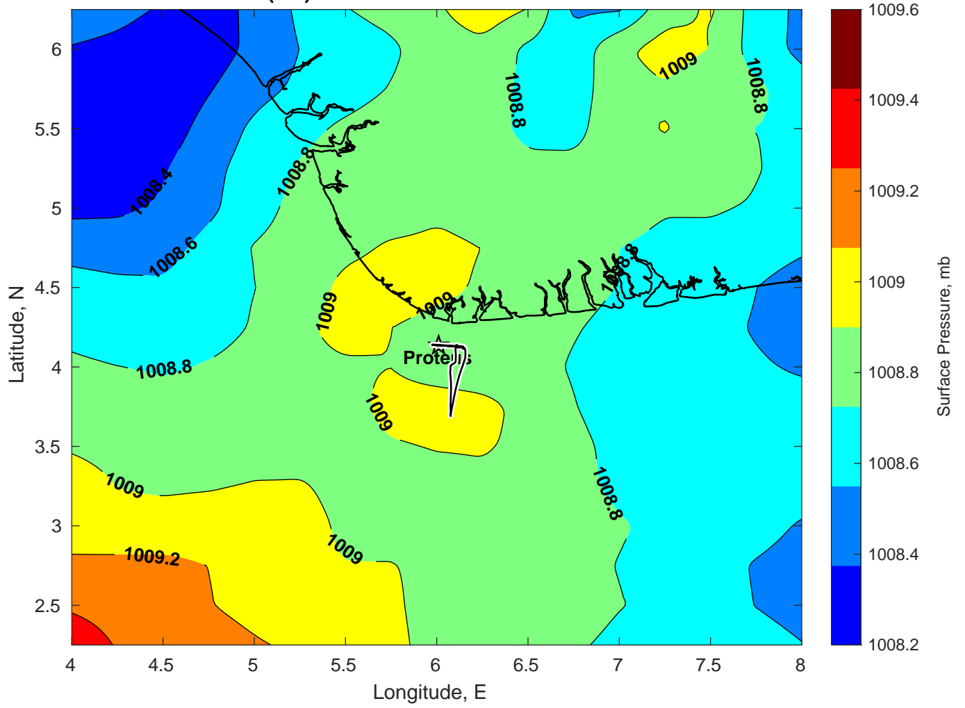
Surface Pressure (mb) for Proteus at 13-Feb-2025 00:00:00
