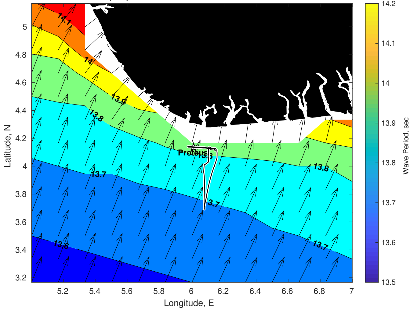
Wave Period (sec) for Proteus at 13-Feb-2025 09:00:00
