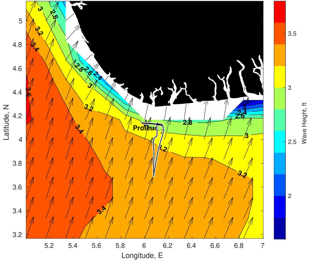
Wave Height (ft) for Proteus at 13-Feb-2025 09:00:00
