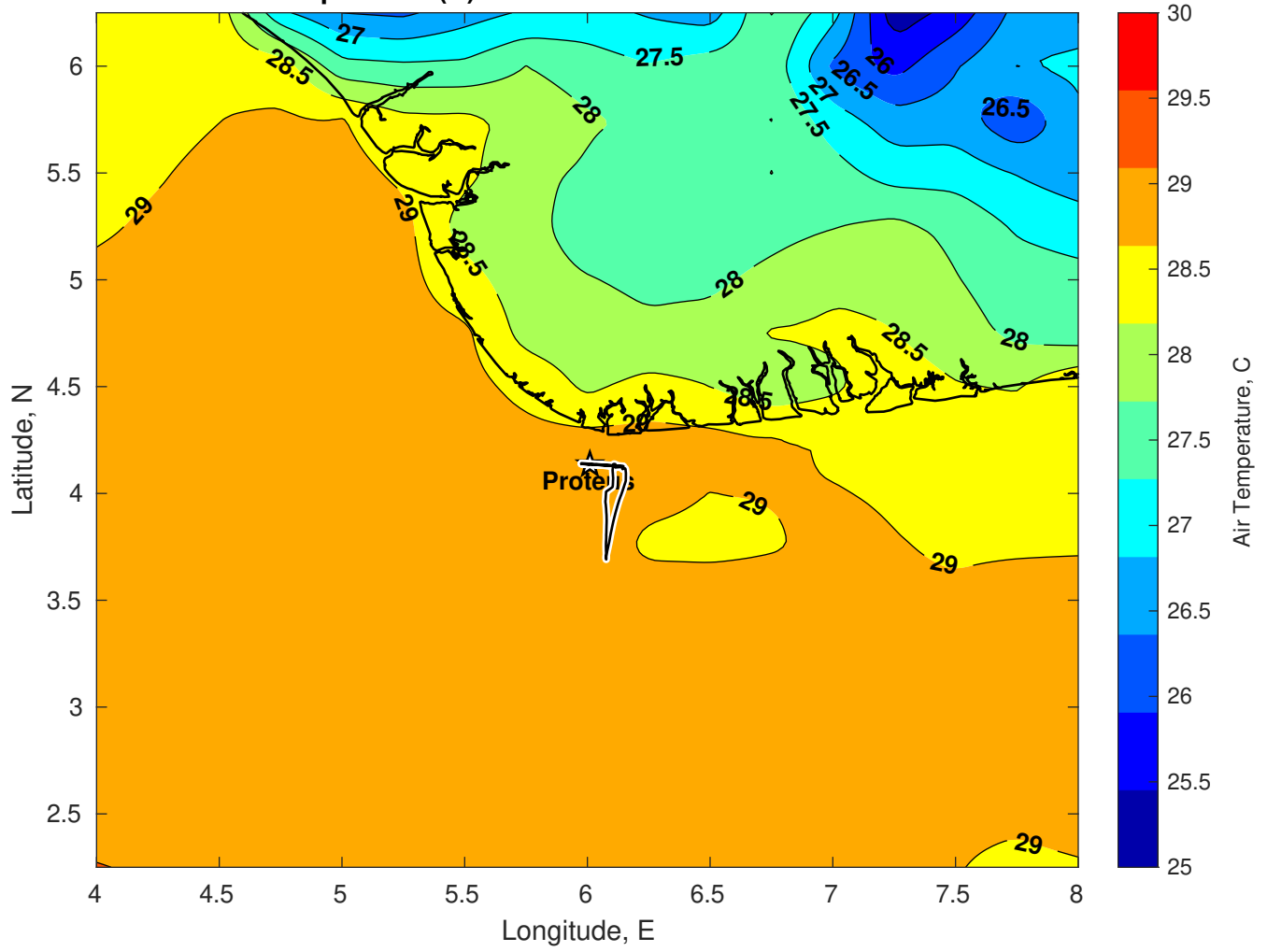
Air Temperature (C) for Proteus at 13-Feb-2025
