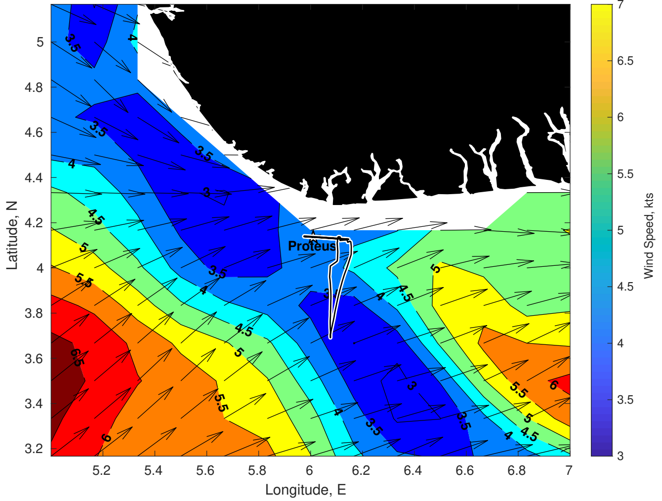
Winds (kts) for Proteus at 13-Feb-2025 09:00:00
