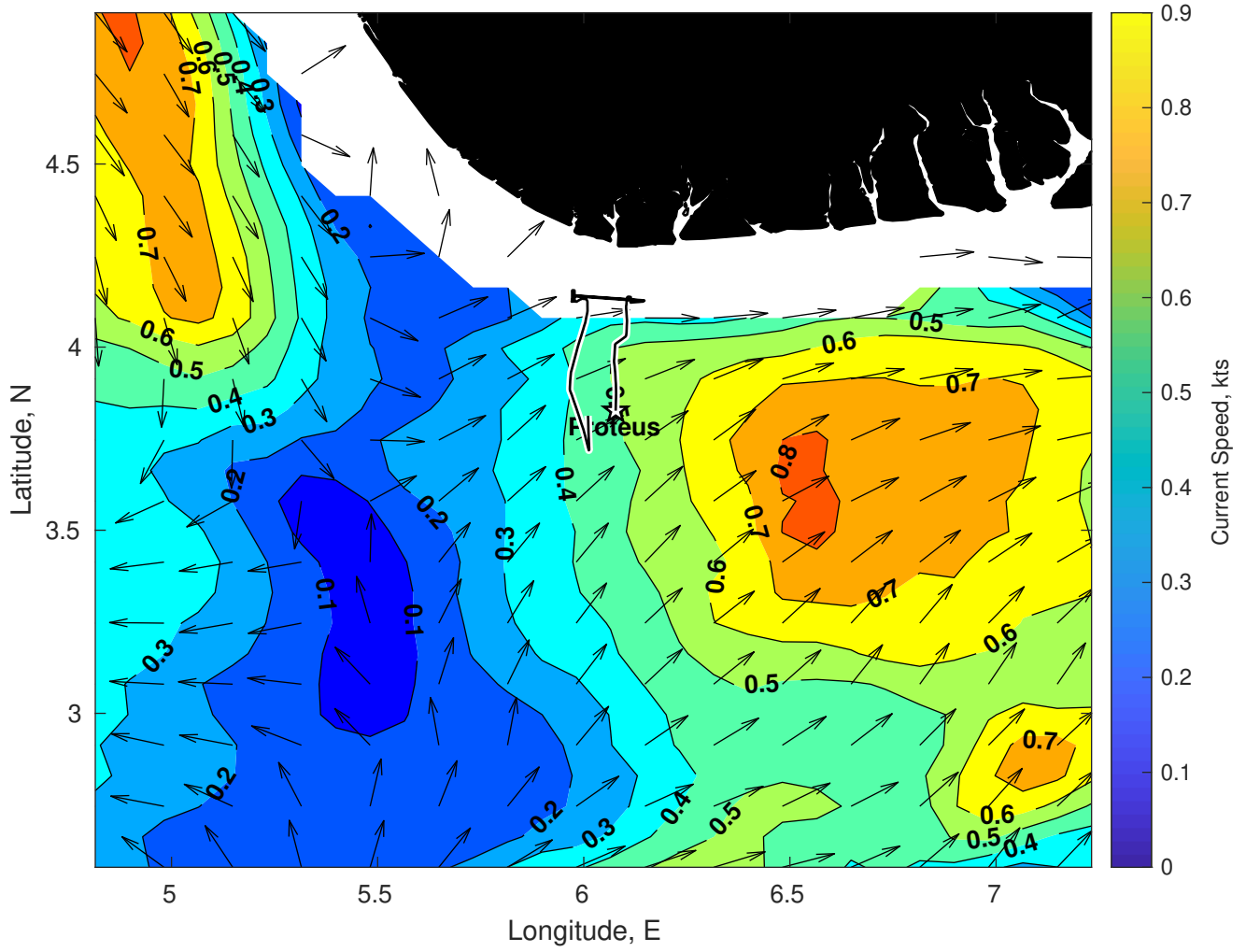
Surface Currents for Proteus at 12-Feb-2025 00:00:00
