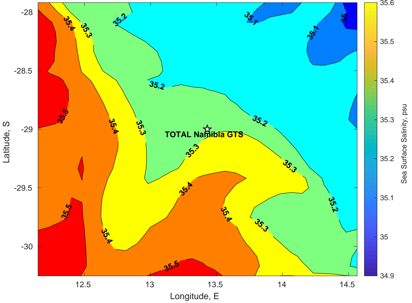
Surface Salinity for TOTAL Namibia GTS at 12-Feb-2025 00:00:00
