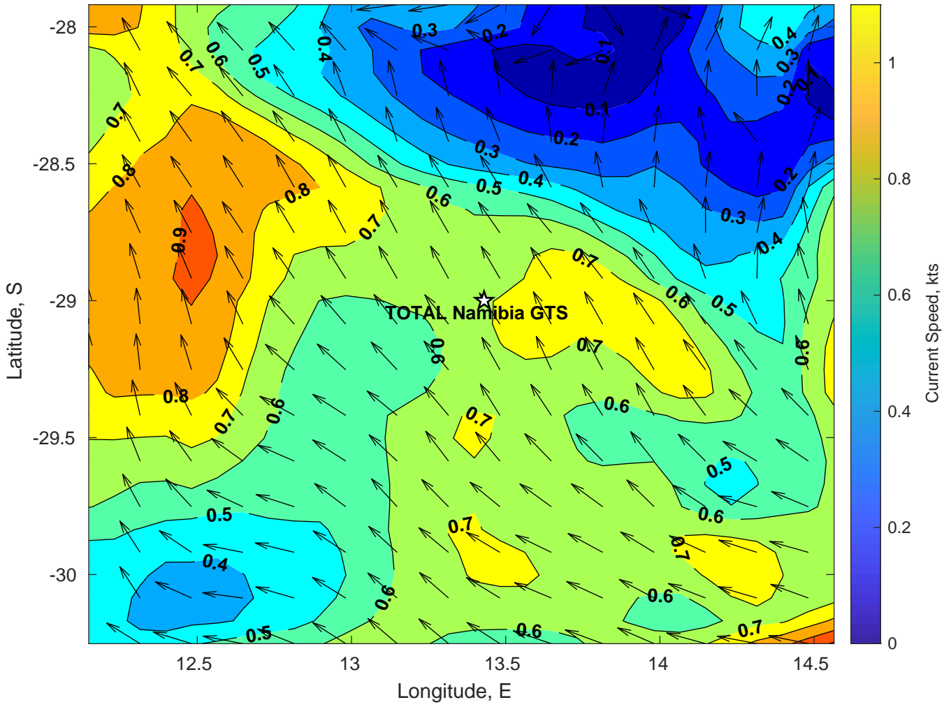
Surface Currents for TOTAL Namibia GTS at 12-Feb-2025 00:00:00
