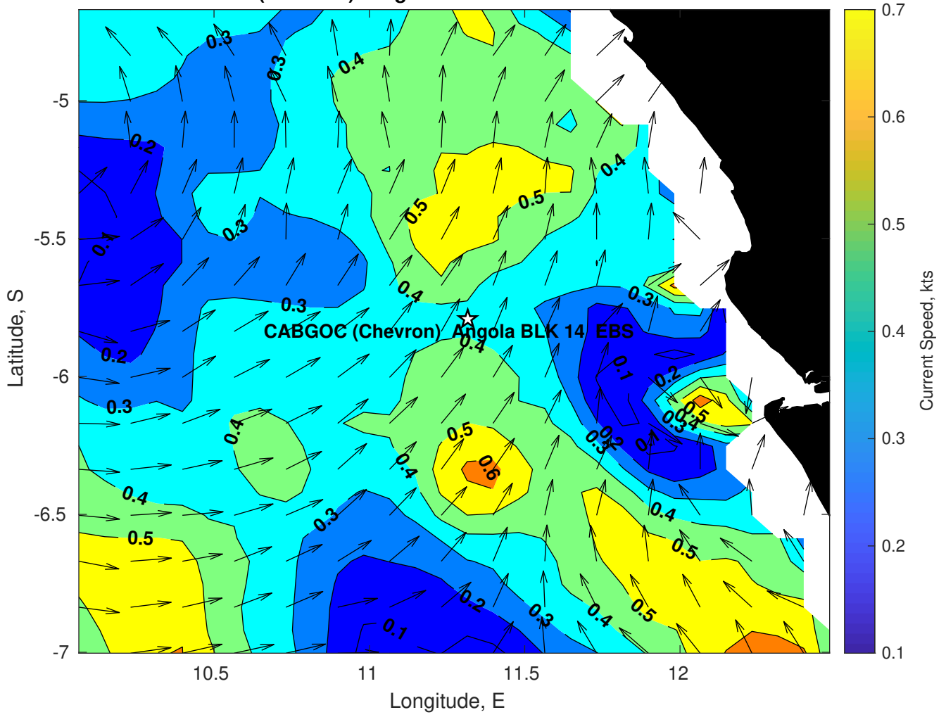
Surface Currents for CABGOC (Chevron) Angola BLK 14 EBS at 13-Feb-2025 00:00:00
