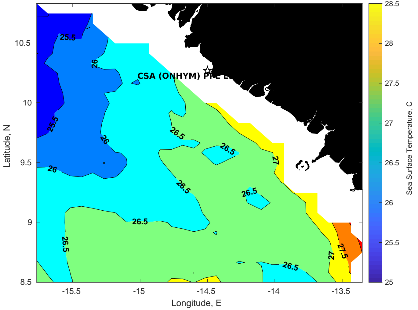
SST for CSA (ONHYM) PPL EBS - Guinea at 13-Feb-2025 00:00:00
