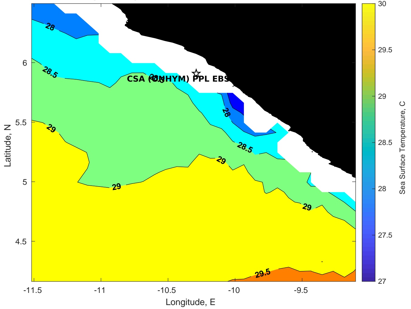
SST for CSA (ONHYM) PPL EBS - Liberia at 13-Feb-2025 00:00:00
