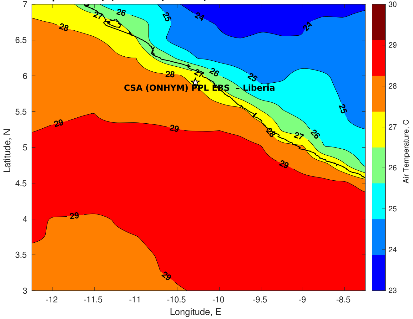
Air Temperature (C) for CSA (ONHYM) PPL EBS - Liberia at 14-Feb-2025
