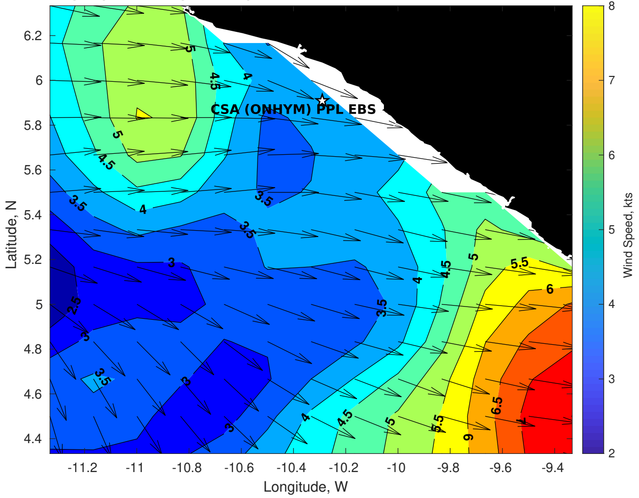
Winds (kts) for CSA (ONHYM) PPL EBS - Liberia at 13-Feb-2025 09:00:00
