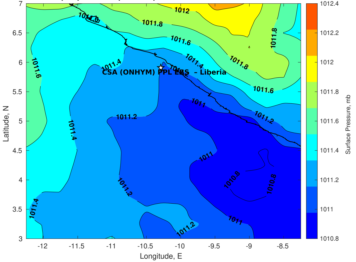
Surface Pressure (mb) for CSA (ONHYM) PPL EBS - Liberia at 14-Feb-2025 00:00:00
