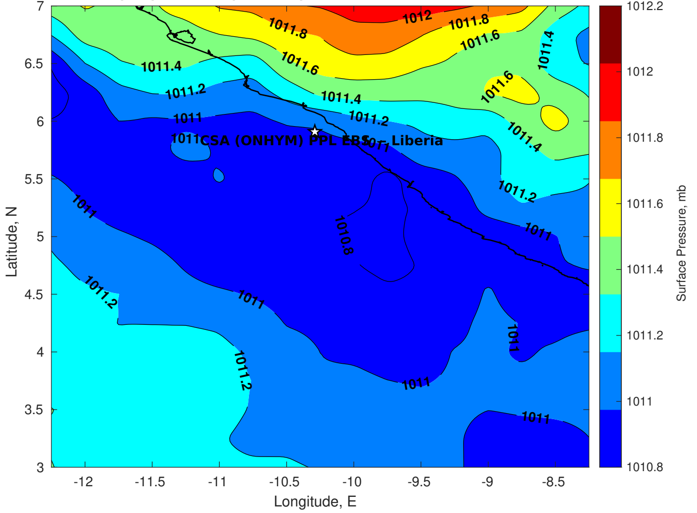
Surface Pressure (mb) for CSA (ONHYM) PPL EBS - Liberia at 15-Feb-2025 00:00:00
