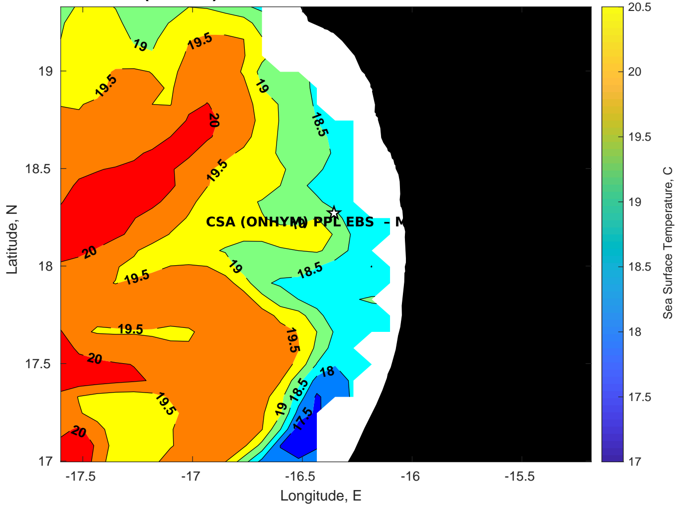
SST for CSA (ONHYM) PPL EBS - Mauritania at 13-Feb-2025 00:00:00
