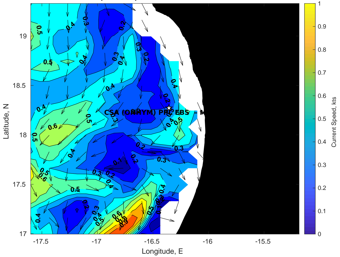
Surface Currents for CSA (ONHYM) PPL EBS - Mauritania at 13-Feb-2025 00:00:00
