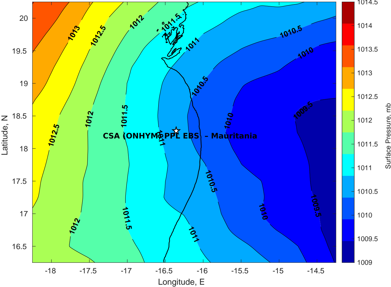
Surface Pressure (mb) for CSA (ONHYM) PPL EBS - Mauritania at 14-Feb-2025 00:00:00
