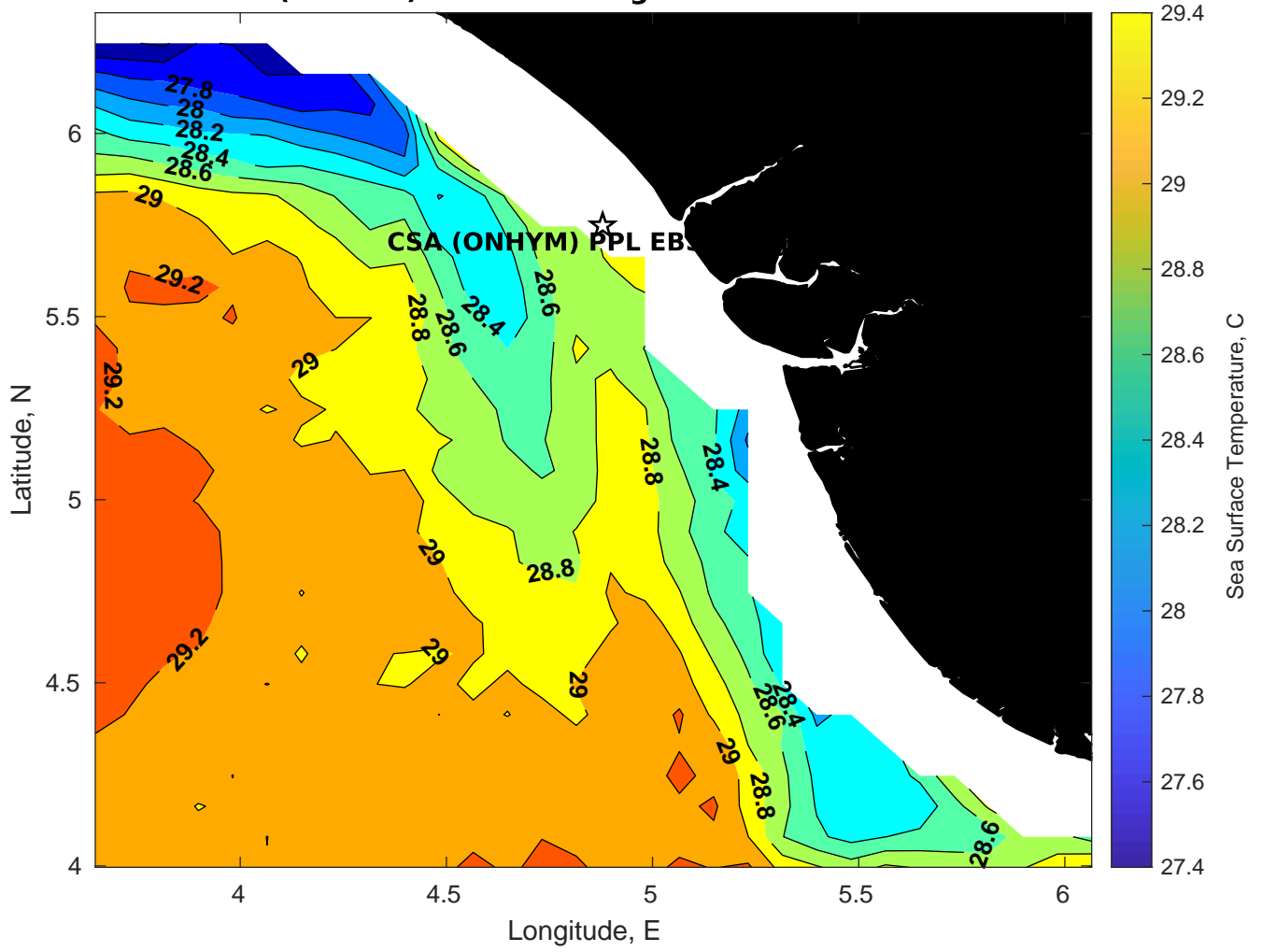
SST for CSA (ONHYM) PPL EBS - Nigeria at 13-Feb-2025 00:00:00
