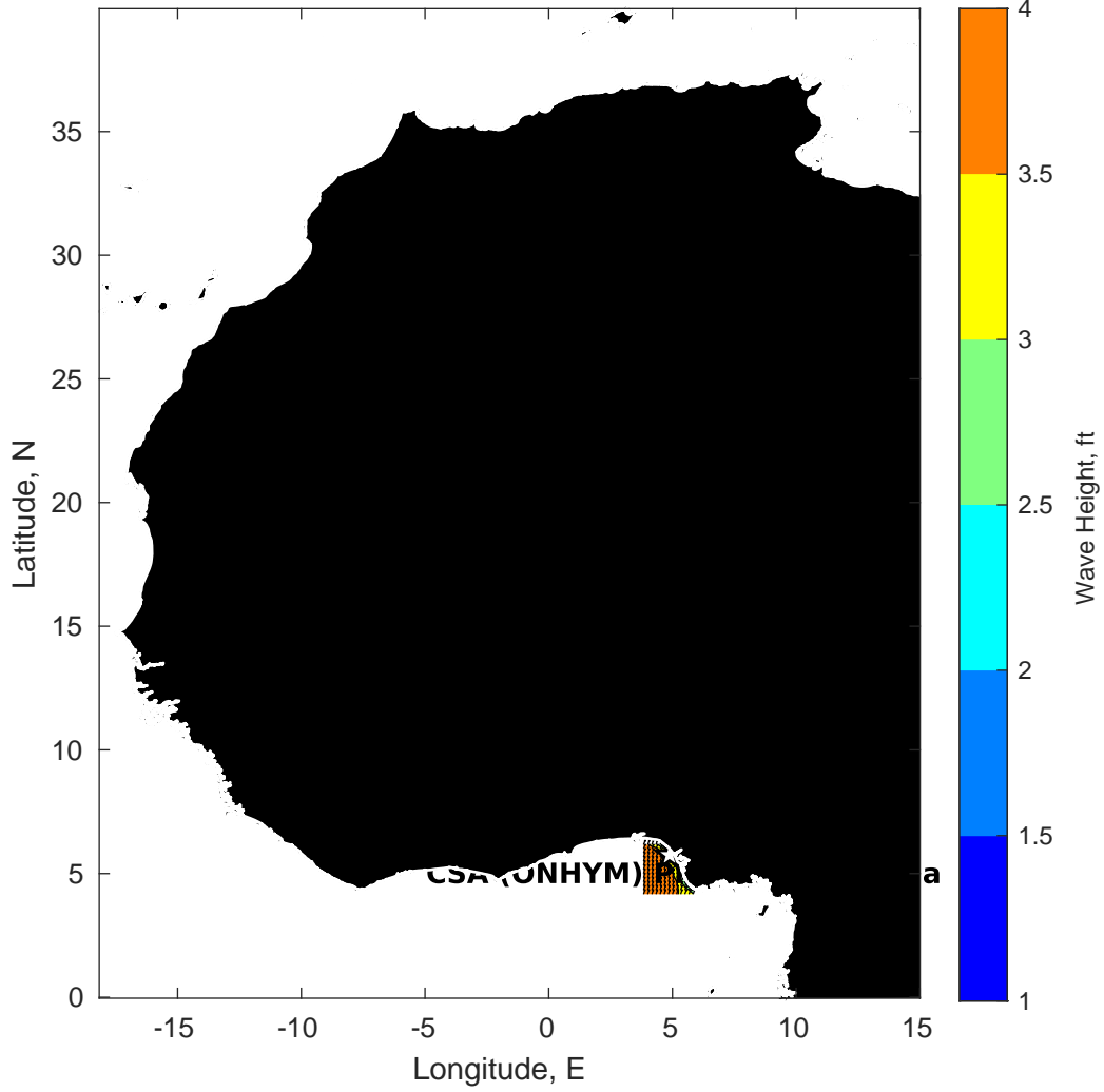
Wave Height (ft) for CSA (ONHYM) PPL EBS - Nigeria at 14-Feb-2025 09:00:00
