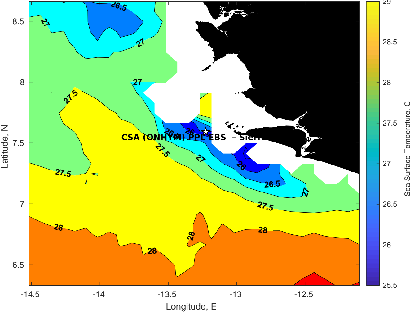
SST for CSA (ONHYM) PPL EBS - Sierra Leone at 13-Feb-2025 00:00:00
