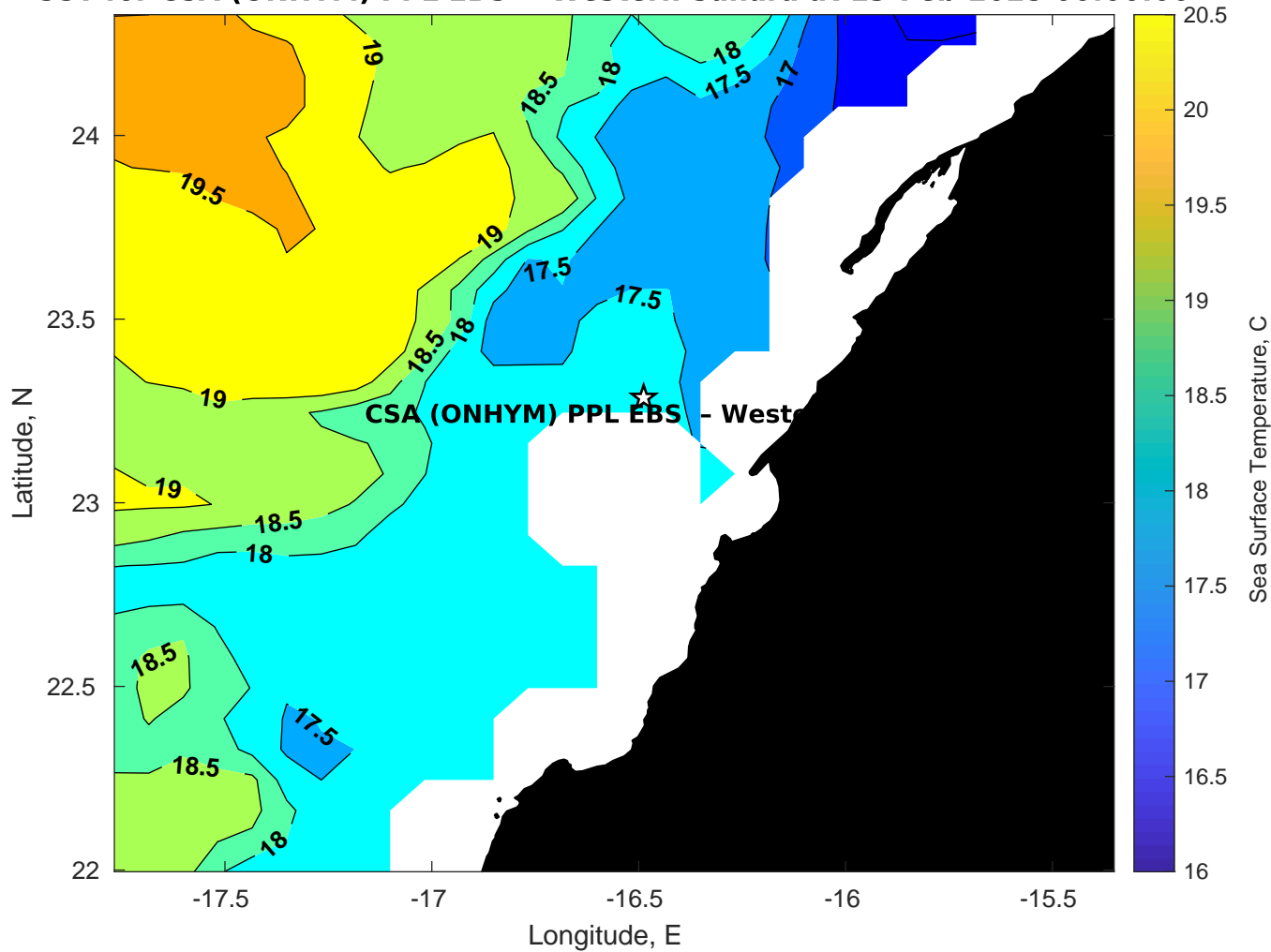
SST for CSA (ONHYM) PPL EBS - Western Sahara at 13-Feb-2025 00:00:00
