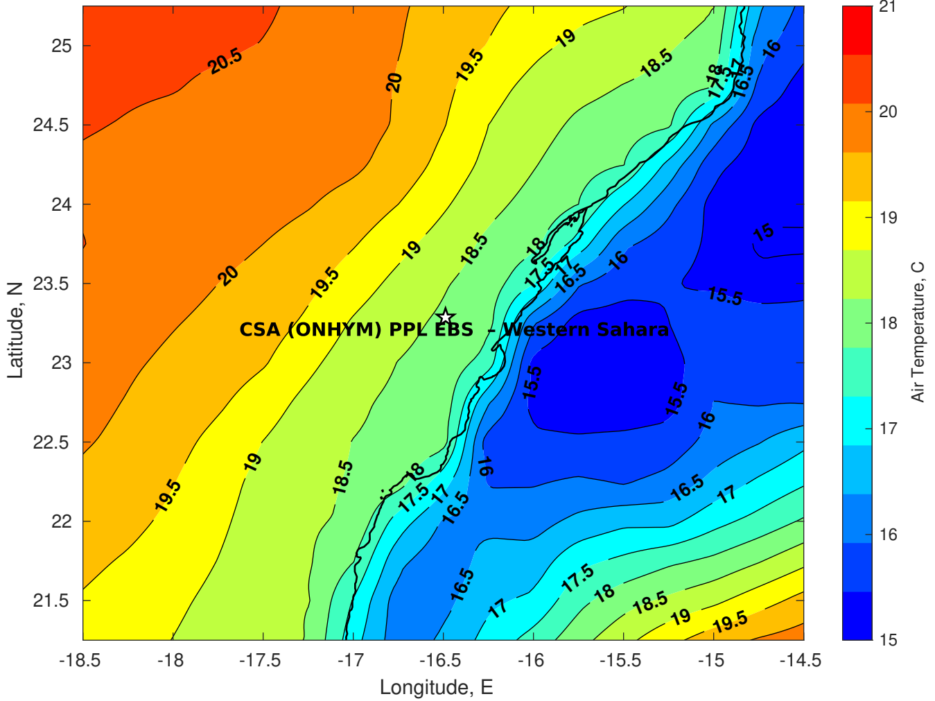
Air Temperature (C) for CSA (ONHYM) PPL EBS - Western Sahara at 14-Feb-2025
