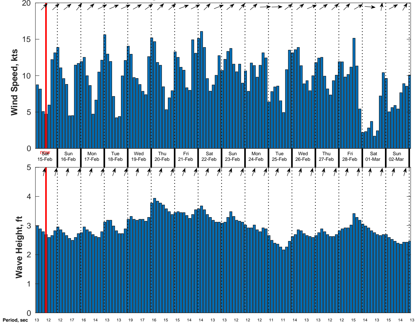
Wind & Wave Forecast for CSL Shell Nigeria from 14-Feb-2025 02:00:00 to 02-Mar-2025 02:00:00
