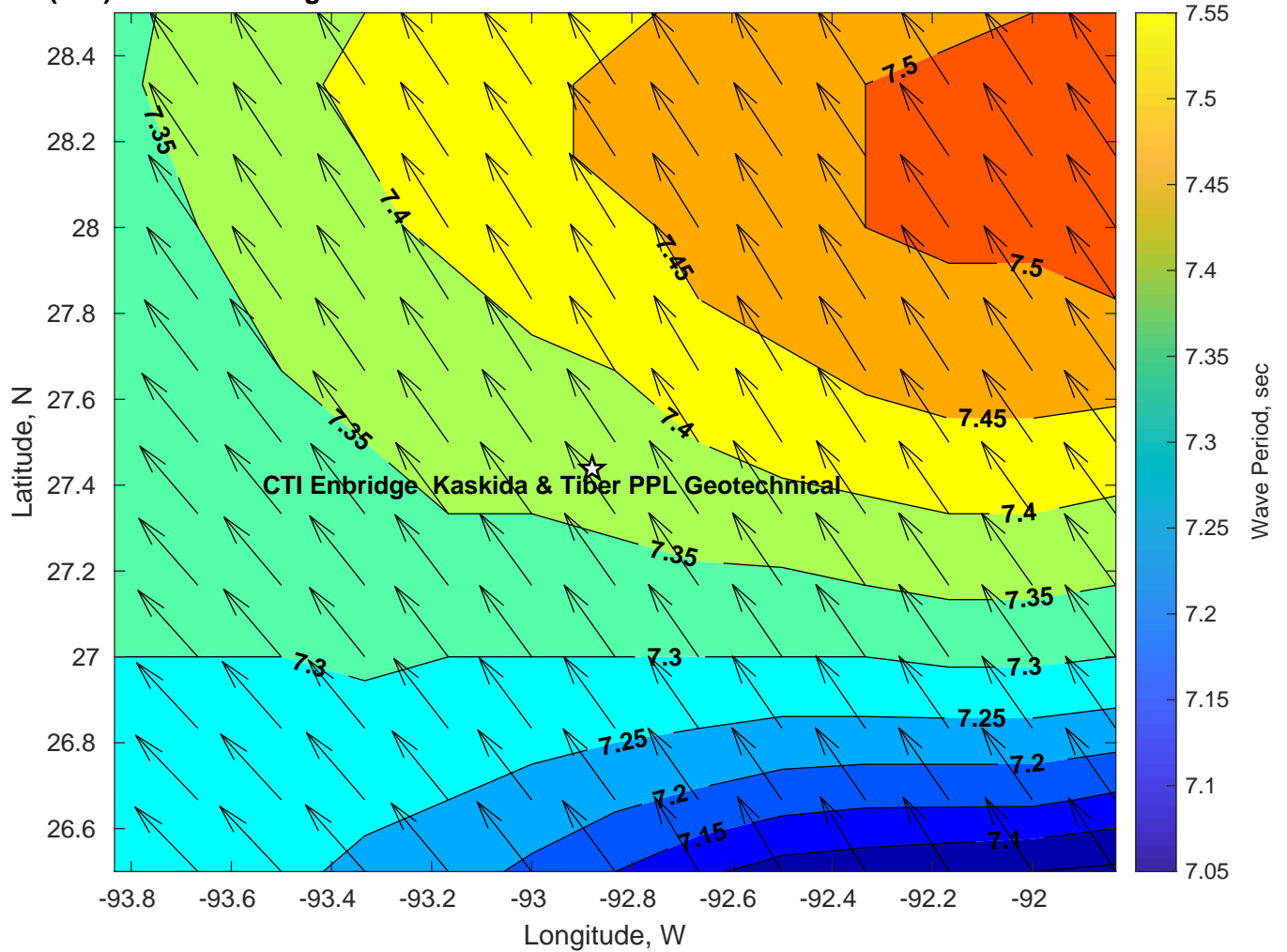
Wave Period (sec) for CTI Enbridge Kaskida & Tiber PPL Geotechnical at 13-Feb-2025 09:00:00
