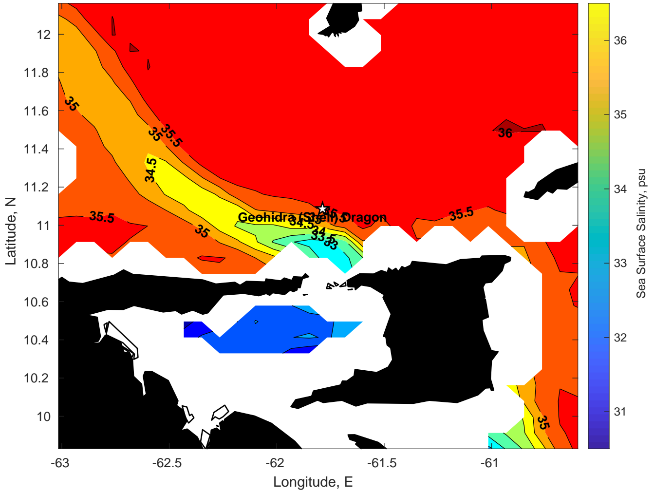
Surface Salinity for Geohidra (Shell) Dragon at 13-Feb-2025 00:00:00
