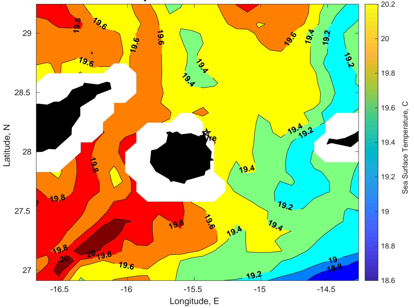
SST for Gyre at 13-Feb-2025 00:00:00
