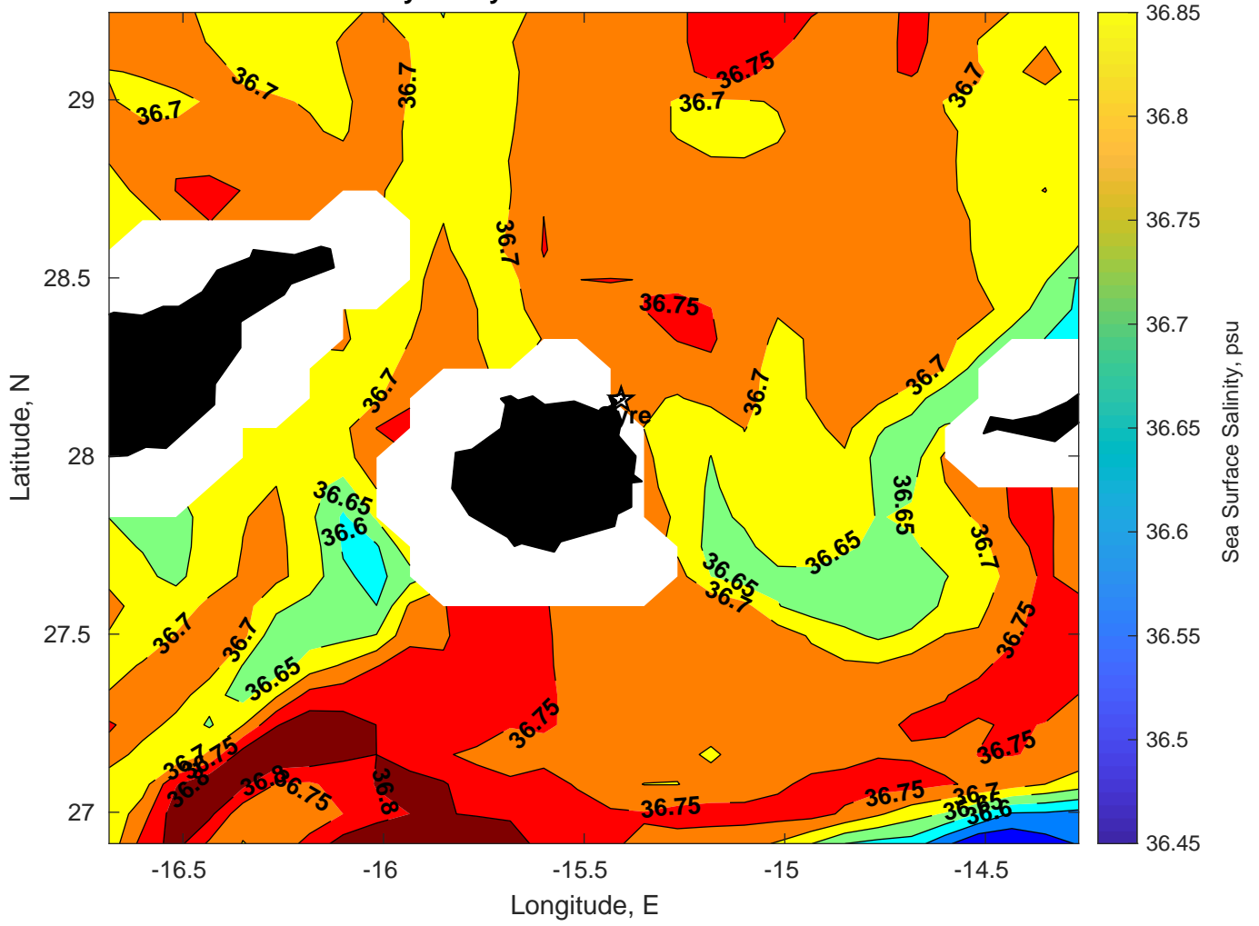
Surface Salinity for Gyre at 13-Feb-2025 00:00:00
