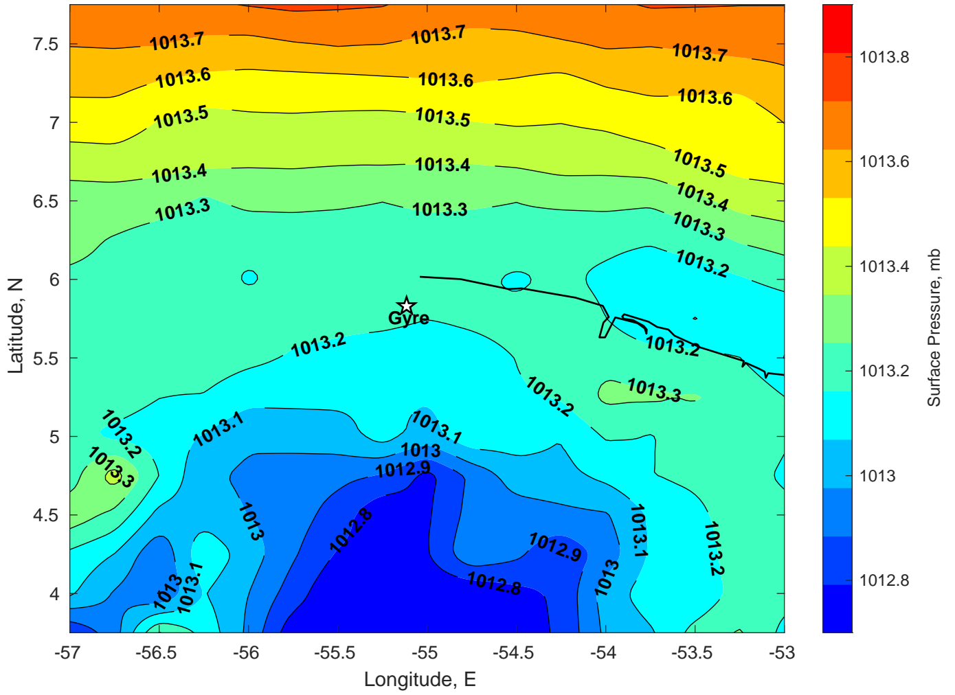
Surface Pressure (mb) for Gyre at 14-Feb-2025 00:00:00
