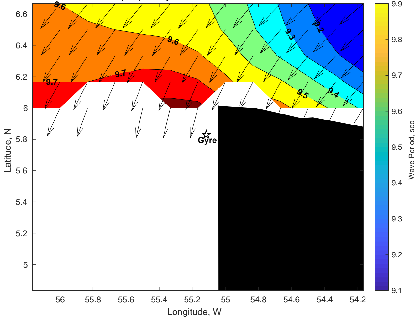
Wave Period (sec) for Gyre at 14-Feb-2025 09:00:00
