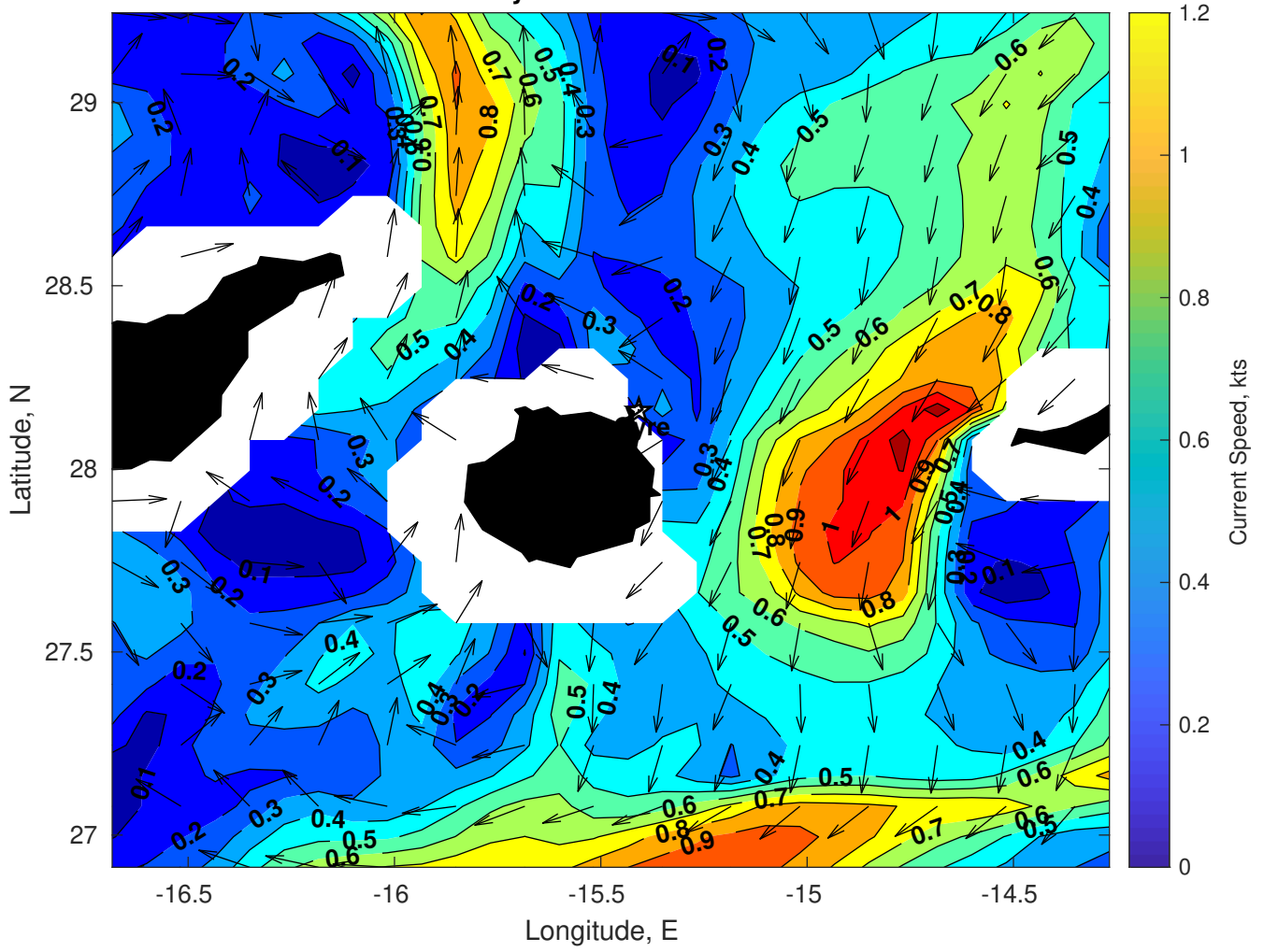
Surface Currents for Gyre at 13-Feb-2025 00:00:00
