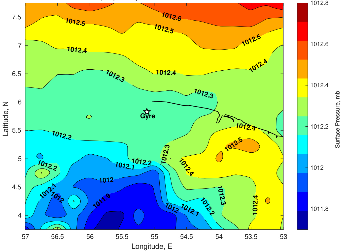
Surface Pressure (mb) for Gyre at 15-Feb-2025 00:00:00
