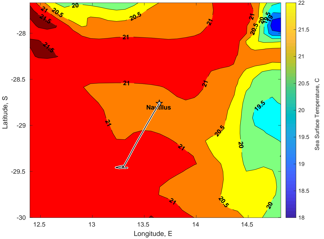
SST for Nautilus at 13-Feb-2025 00:00:00
