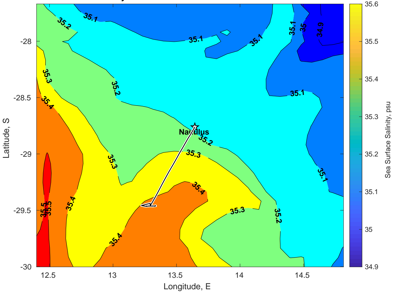
Surface Salinity for Nautilus at 13-Feb-2025 00:00:00
