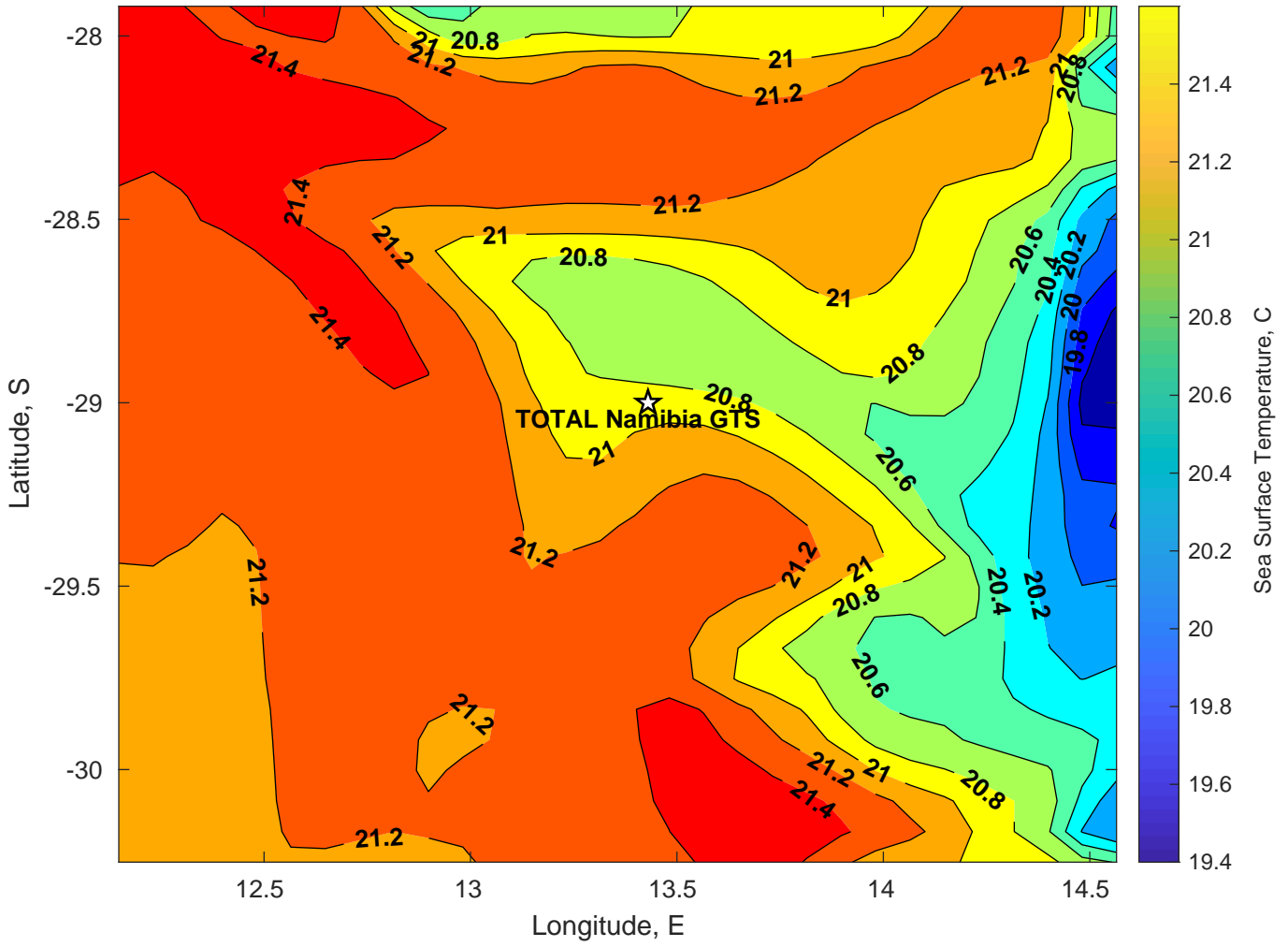
SST for TOTAL Namibia GTS at 13-Feb-2025 00:00:00
