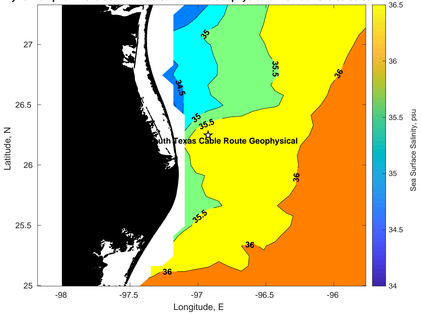
Surface Salinity for Tampnet P2378 South Texas Cable Route Geophysical at 13-Feb-2025 00:00:00
