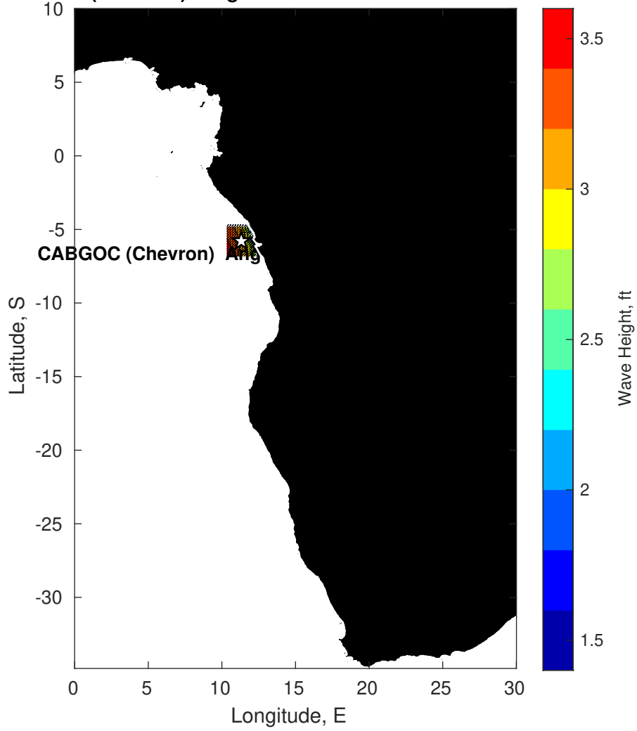
Wave Height (ft) for CABGOC (Chevron) Angola BLK 14 EBS at 15-Feb-2025 09:00:00
