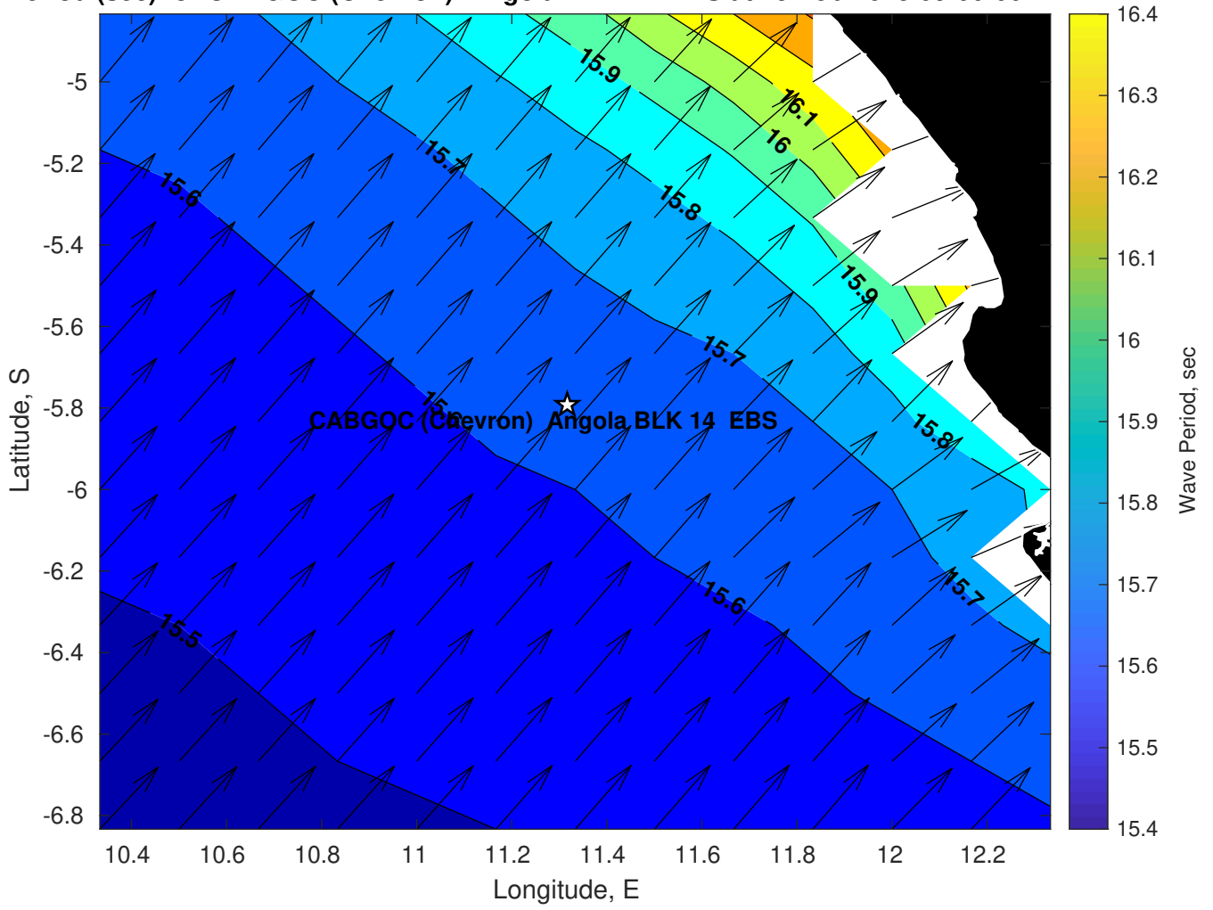
Wave Period (sec) for CABGOC (Chevron) Angola BLK 14 EBS at 15-Feb-2025 09:00:00
