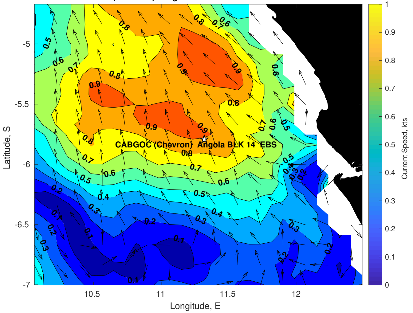
Surface Currents for CABGOC (Chevron) Angola BLK 14 EBS at 14-Feb-2025 00:00:00
