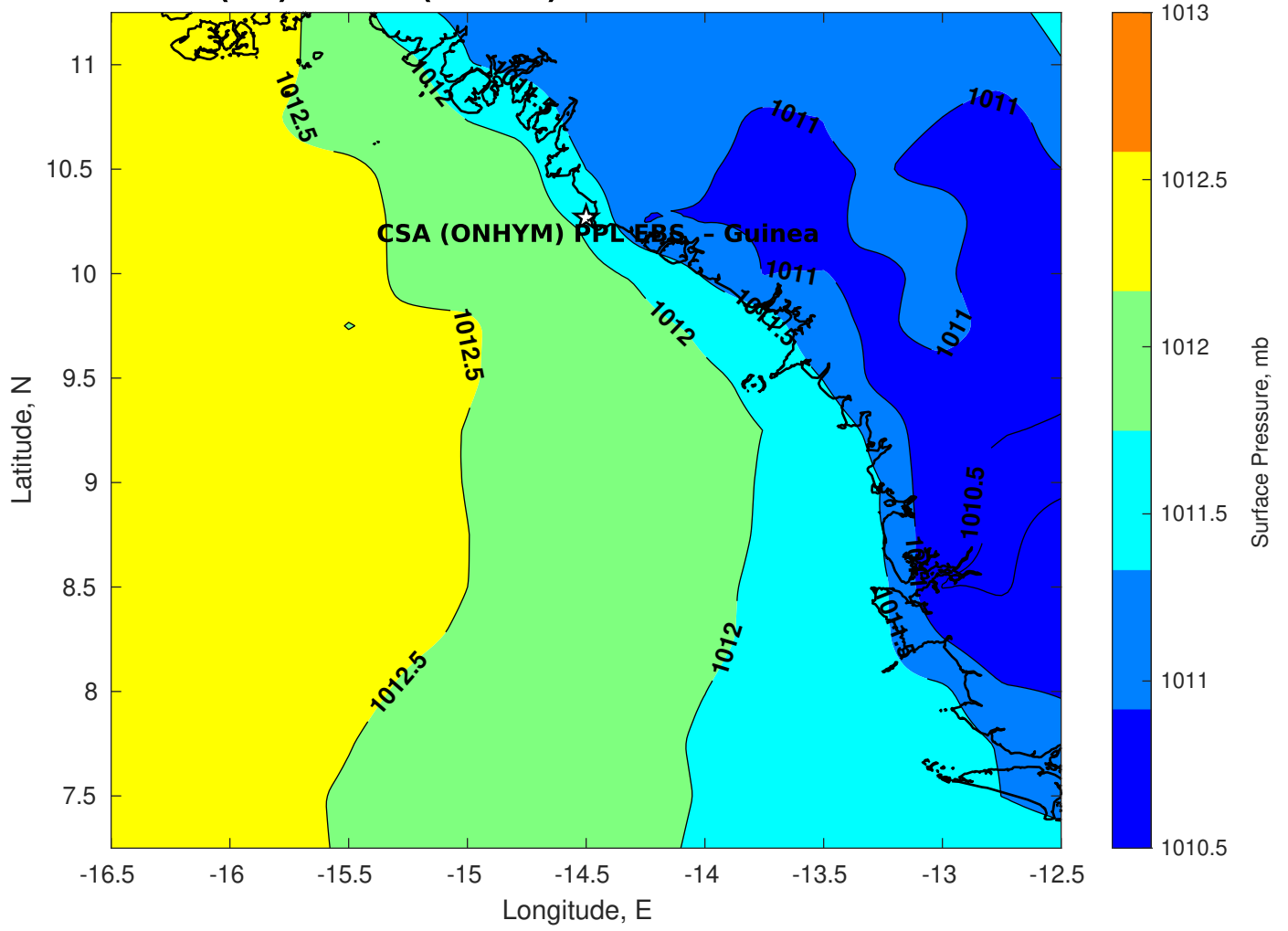
Surface Pressure (mb) for CSA (ONHYM) PPL EBS - Guinea at 15-Feb-2025 12:00:00
