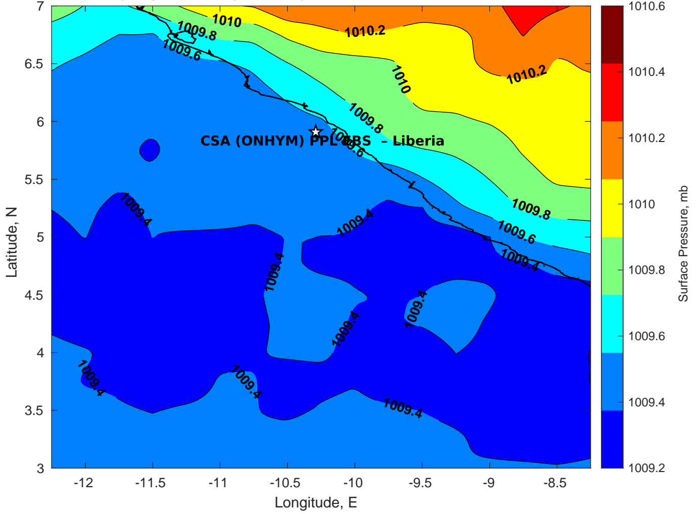
Surface Pressure (mb) for CSA (ONHYM) PPL EBS - Liberia at 15-Feb-2025 06:00:00
