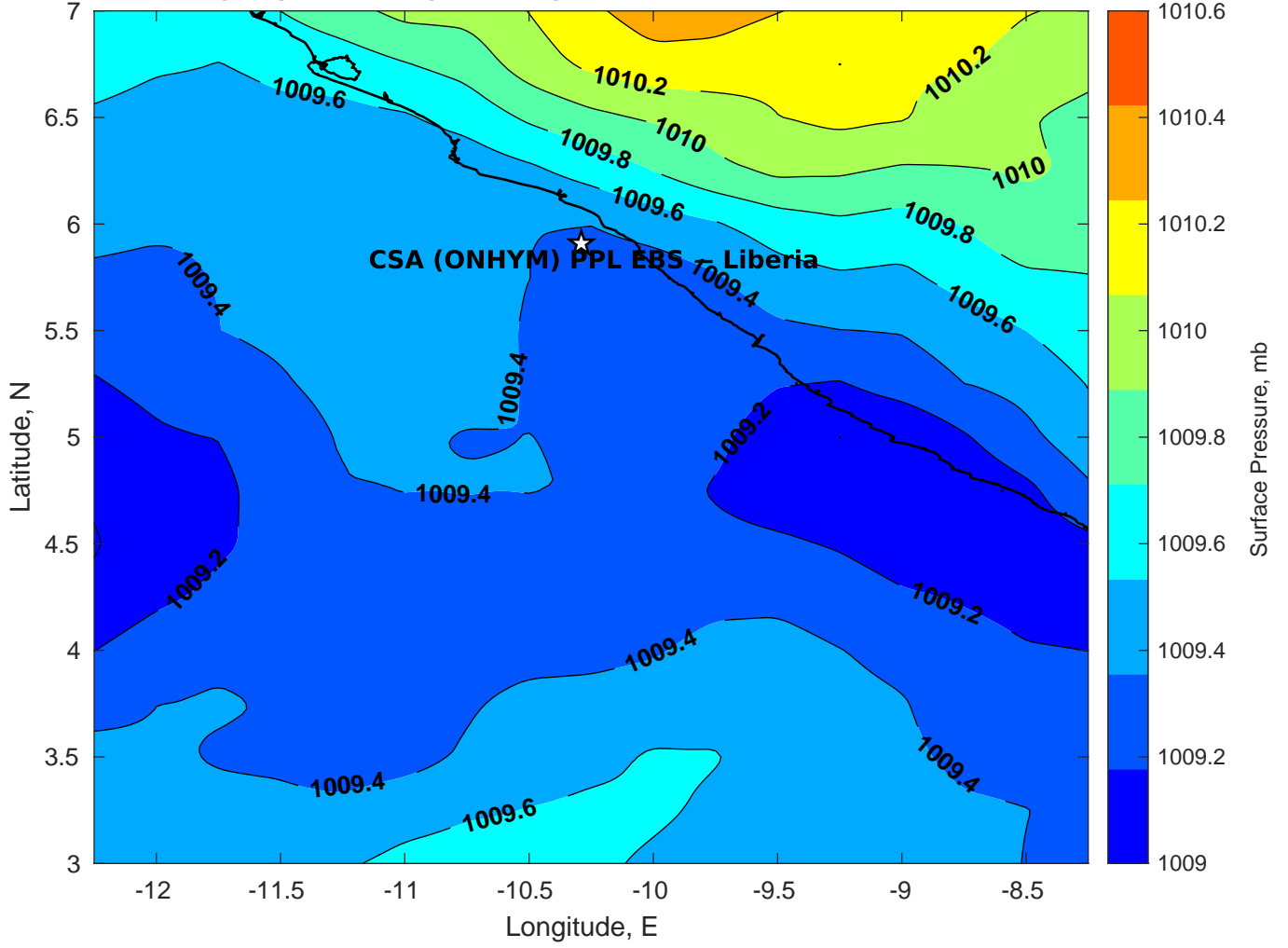
Surface Pressure (mb) for CSA (ONHYM) PPL EBS - Liberia at 17-Feb-2025 06:00:00
