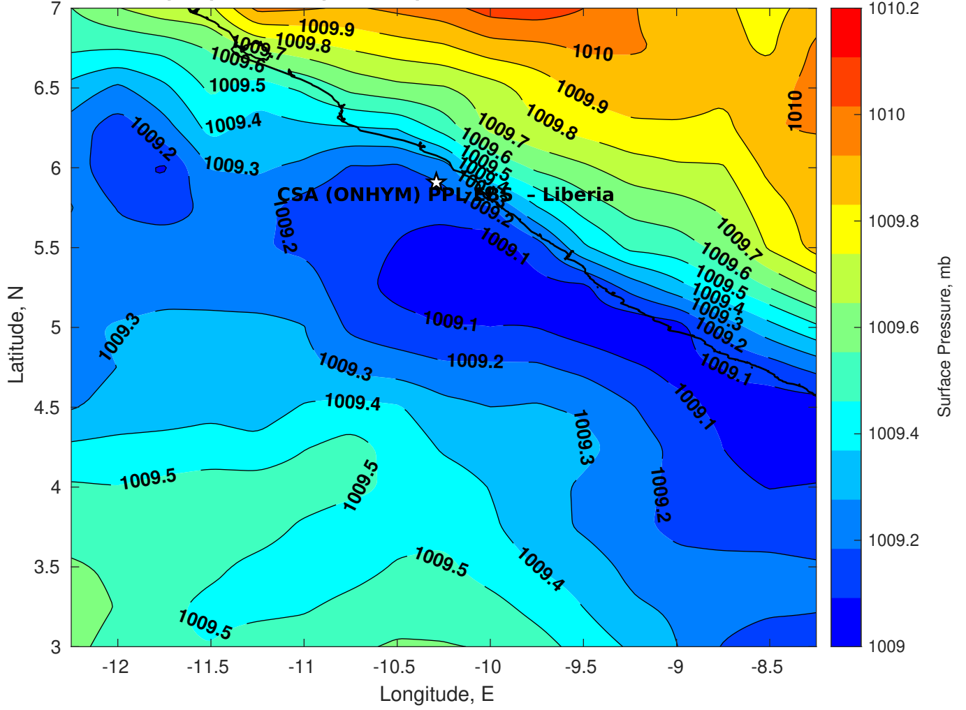
Surface Pressure (mb) for CSA (ONHYM) PPL EBS - Liberia at 16-Feb-2025 06:00:00
