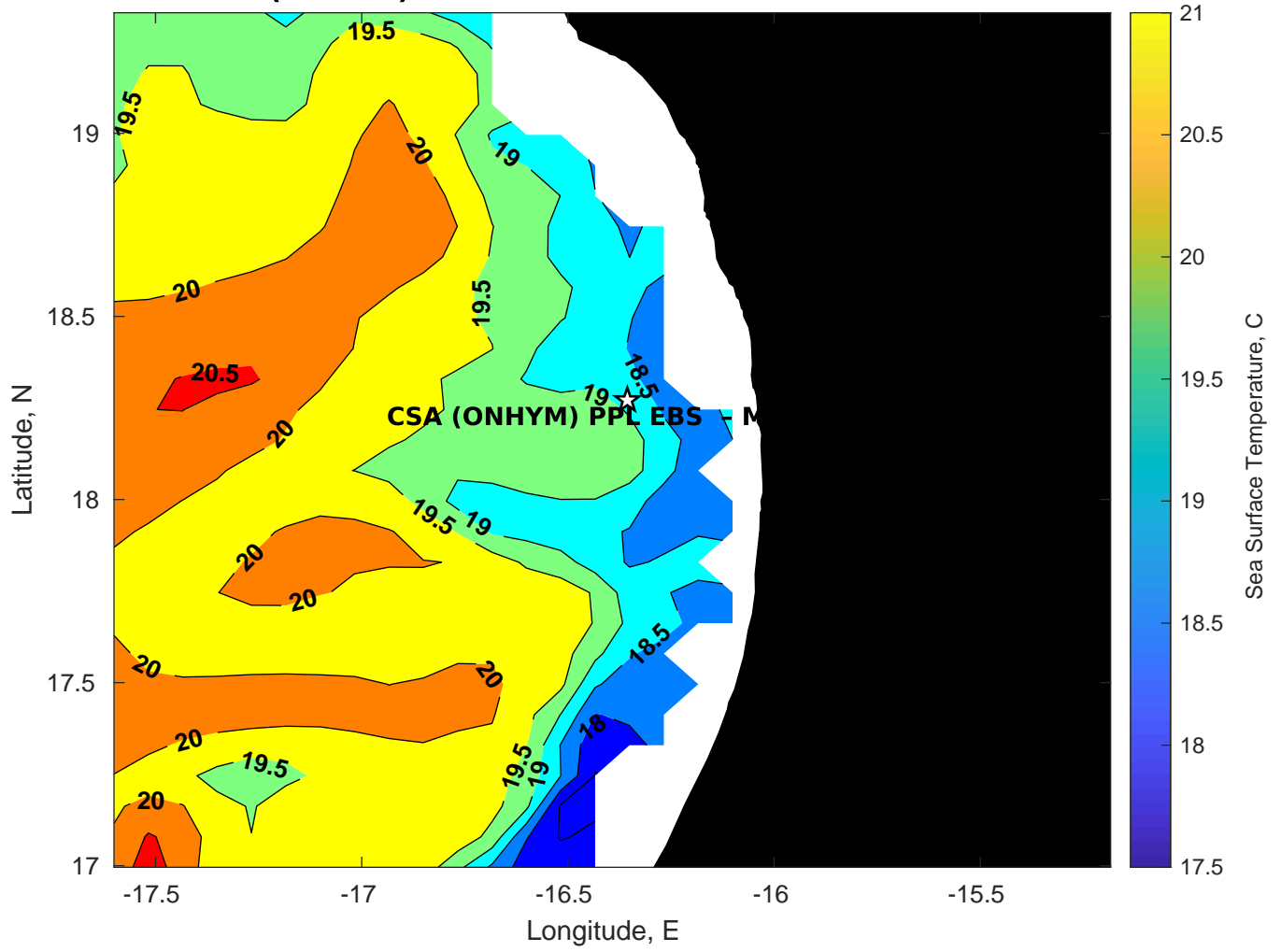
SST for CSA (ONHYM) PPL EBS - Mauritania at 14-Feb-2025 00:00:00
