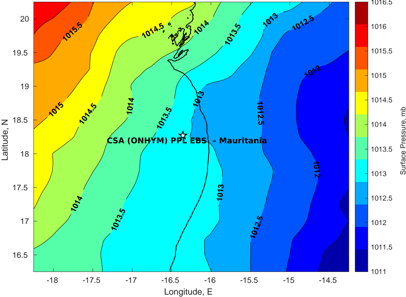
Surface Pressure (mb) for CSA (ONHYM) PPL EBS - Mauritania at 16-Feb-2025 00:00:00
