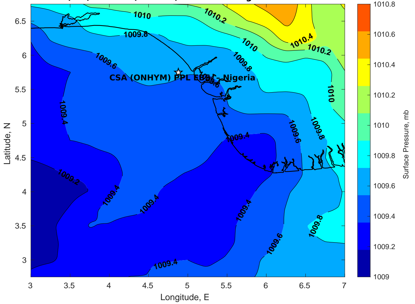
Surface Pressure (mb) for CSA (ONHYM) PPL EBS - Nigeria at 15-Feb-2025 06:00:00
