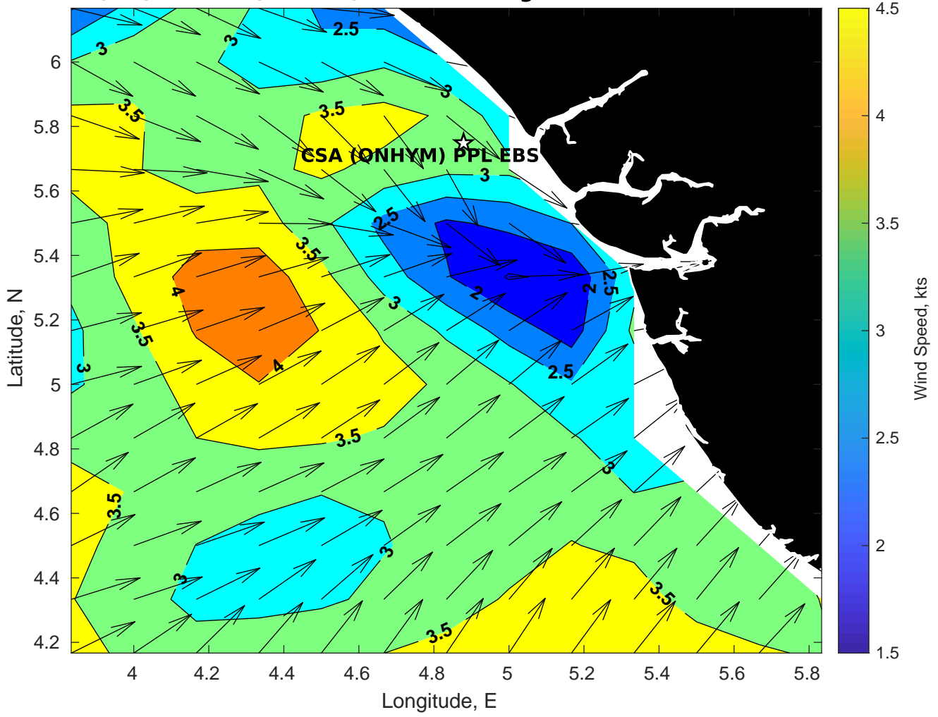
Winds (kts) for CSA (ONHYM) PPL EBS - Nigeria at 15-Feb-2025 09:00:00
