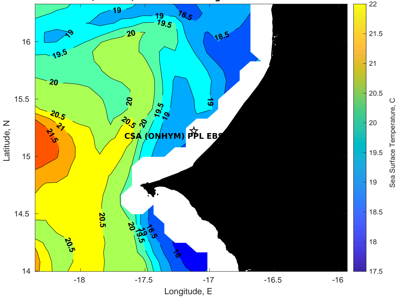
SST for CSA (ONHYM) PPL EBS - Senegal at 14-Feb-2025 00:00:00
