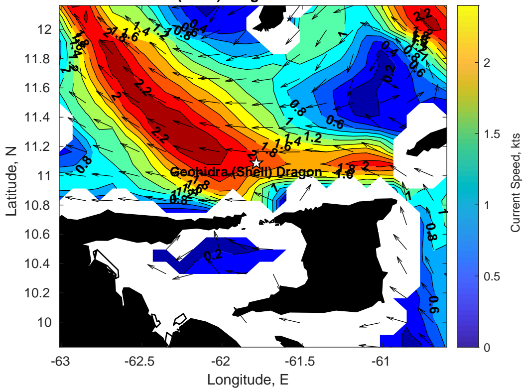
Surface Currents for Geohidra (Shell) Dragon at 14-Feb-2025 00:00:00
