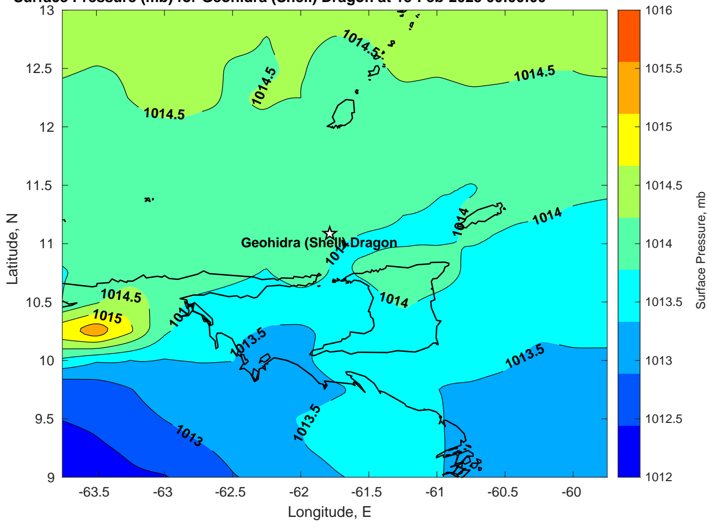
Surface Pressure (mb) for Geohdra (Shell) Dragon at 15-Feb-2025 00:00:00
