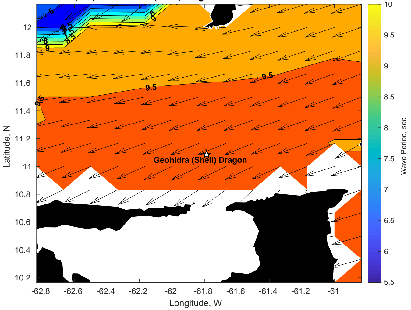
Wave Period (sec) for Geohidra (Shell) Dragon at 15-Feb-2025 09:00:00
