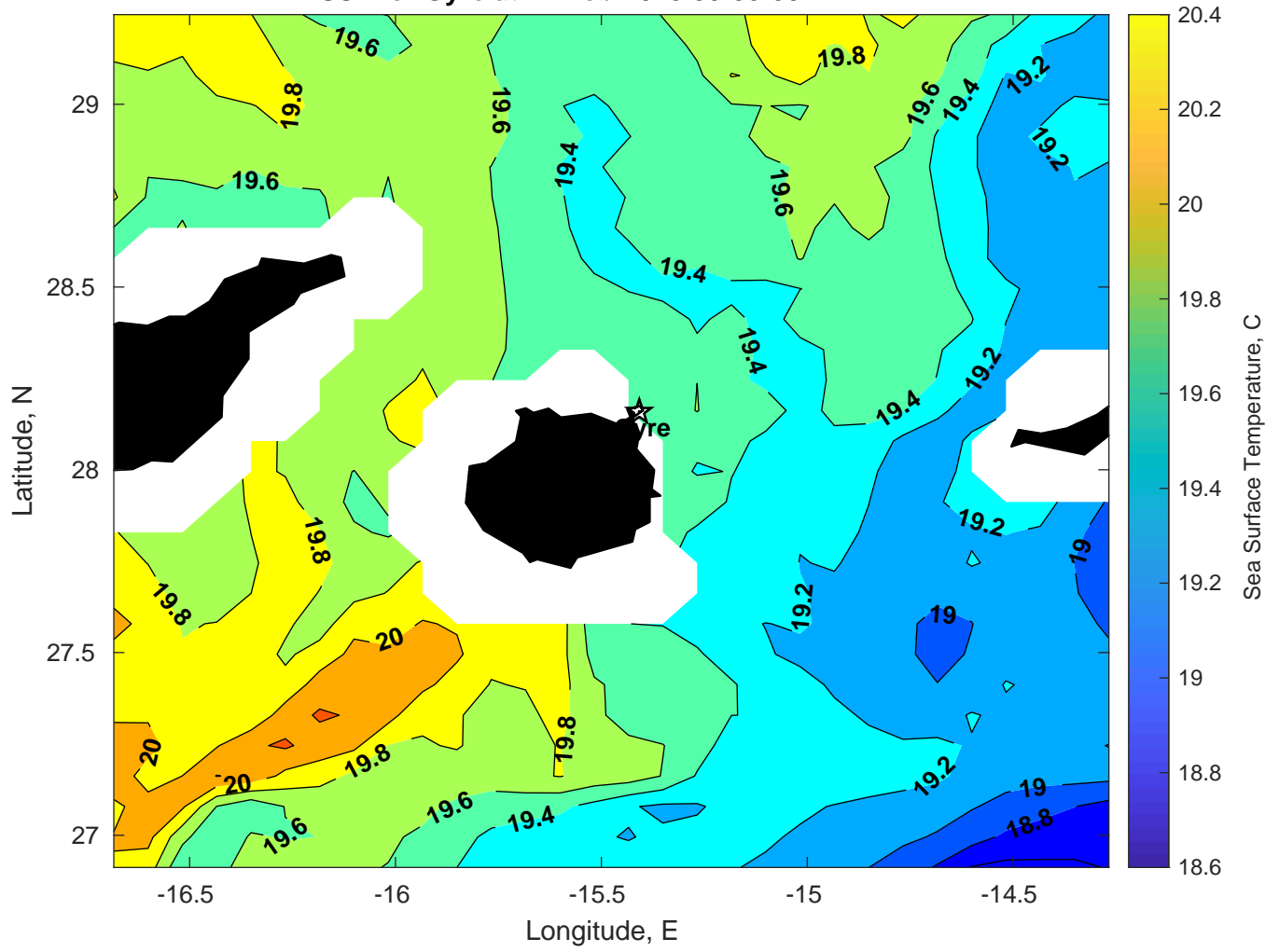
SST for Gyre at 14-Feb-2025 00:00:00
