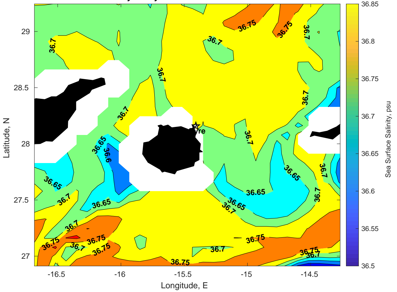
Surface Salinity for Gyre at 14-Feb-2025 00:00:00
