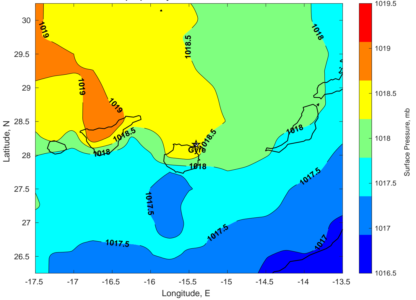
Surface Pressure (mb) for Gyre at 16-Feb-2025 00:00:00
