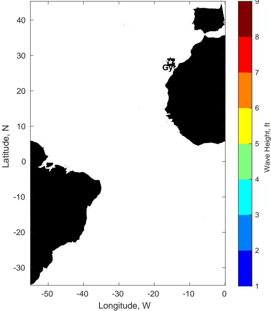
Wave Height (ft) for Gyre at 15-Feb-2025 09:00:00
