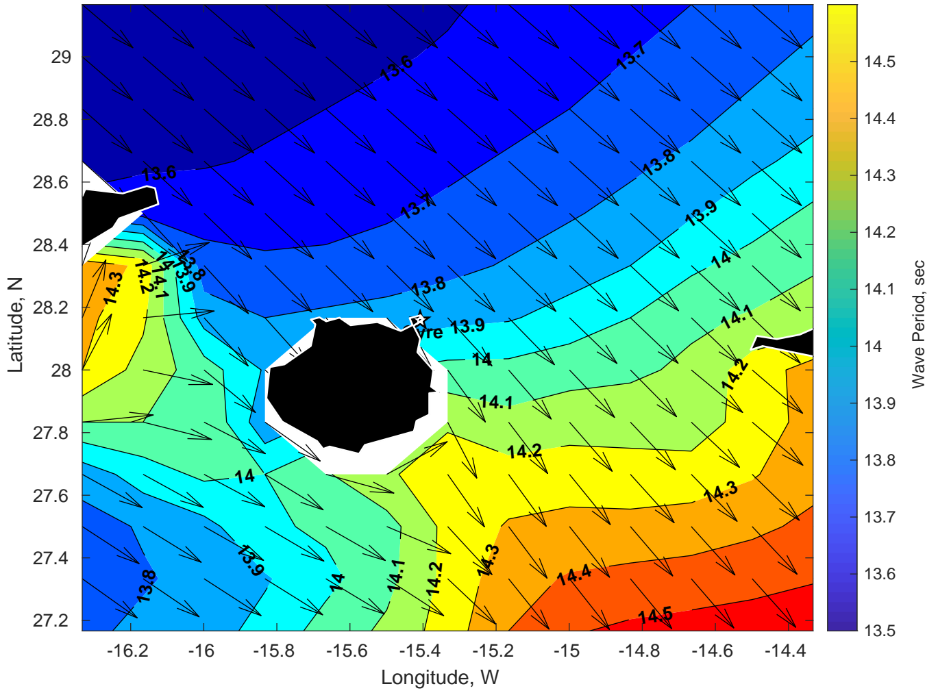
Wave Period (sec) for Gyre at 15-Feb-2025 09:00:00
