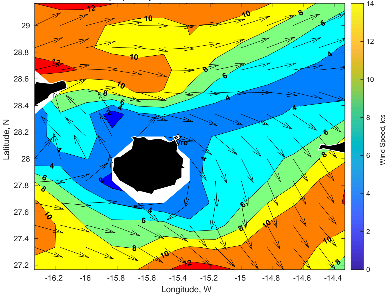
Winds (kts) for Gyre at 15-Feb-2025 09:00:00
