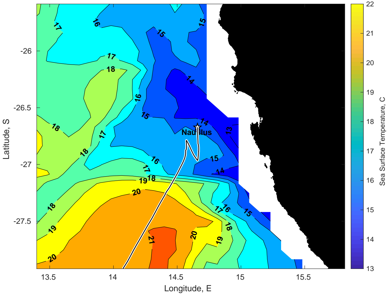
SST for Nautilus at 14-Feb-2025 00:00:00
