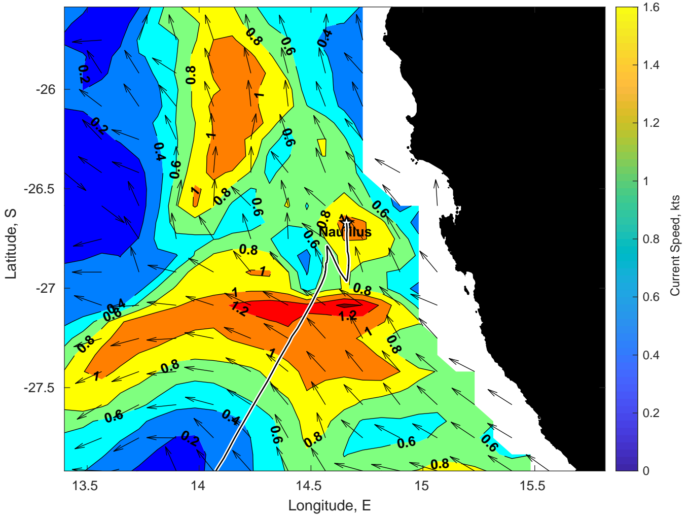
Surface Currents for Nautilus at 14-Feb-2025 00:00:00
