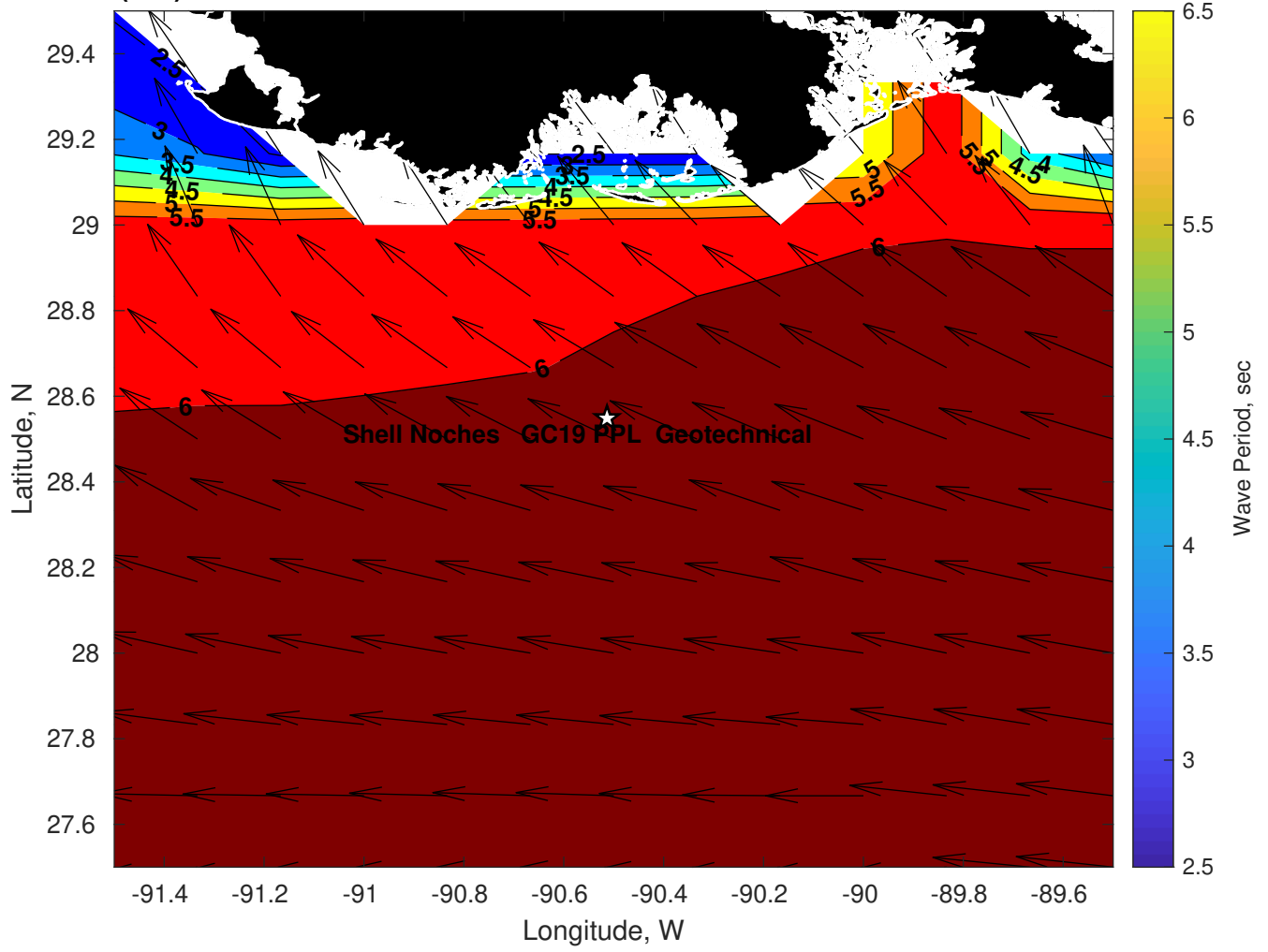
Wave Period (sec) for Shell Noches GC19 PPL Geotechnical at 15-Feb-2025 09:00:00
