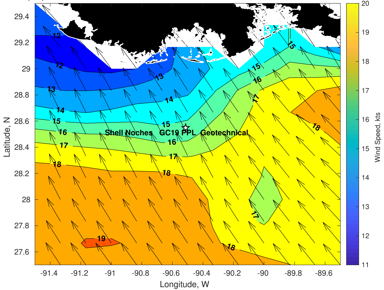
Winds (kts) for Shell Noches GC19 PPL Geotechnical at 15-Feb-2025 09:00:00
